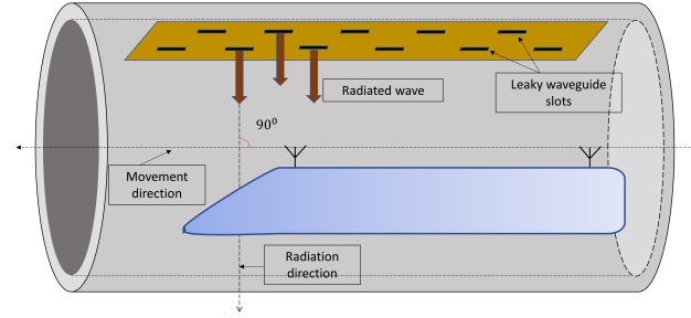
Figure 10: Configuration of the vacuum tube with a leaky waveguide.
