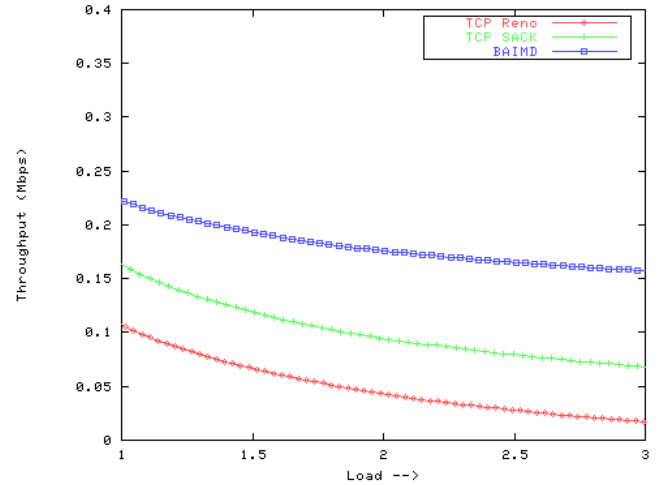
Figure 5. Throughput by TCP Reno, TCP Sack, and BAIMD under high network loads.
