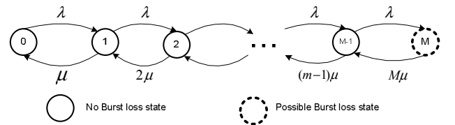
Figure 1. State transition diagram for obtaining burst dropping
