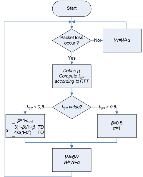
Figure 2. Flow chard demonstrating BAIMD congestion control
