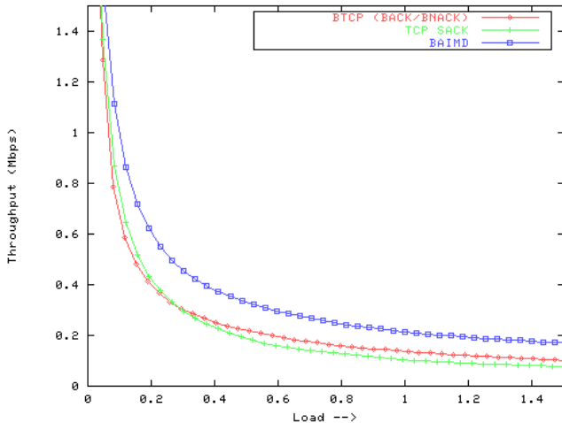
Figure 6. Throughput by BTCP with BACK/BNACK, TCP Sack, and BAIMD scheme.
