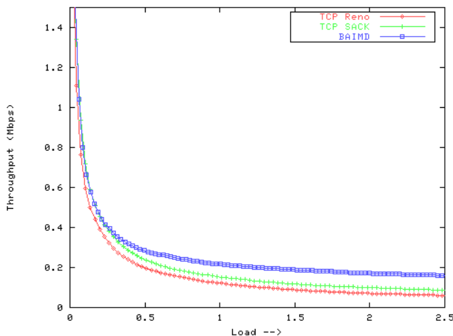
Figure 7. Throughput by the TCP implementations in presence of UDP traffic.
