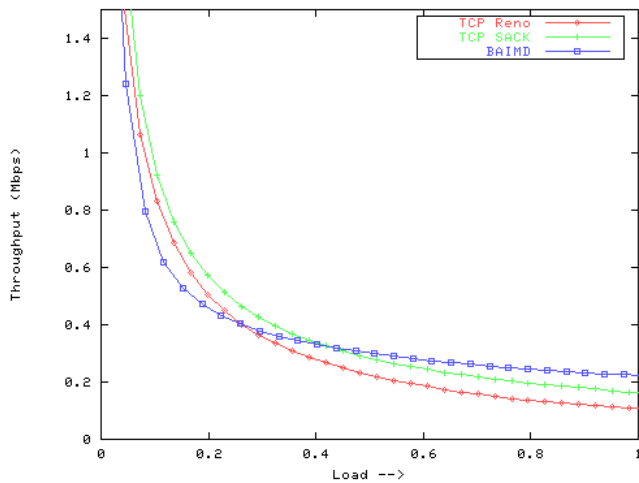
Figure 4. Throughput by TCP Reno, TCP Sack, and BAIMD under low network loads.
