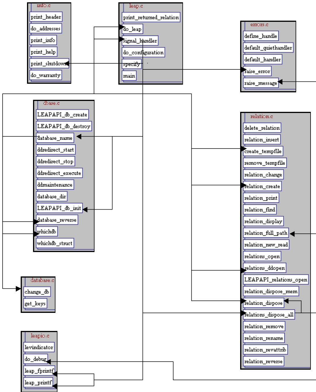
Fig. 4 Signal_handler-to-fuctions calls
