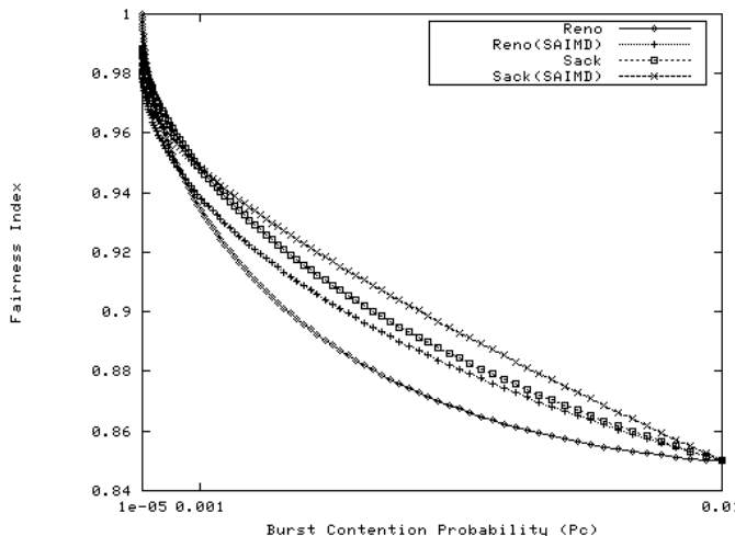
Fig. 13. Fairness Index of Reno, Sack, Reno (SAIMD), and Sack (SAIMD) in a barebone OBS network.
