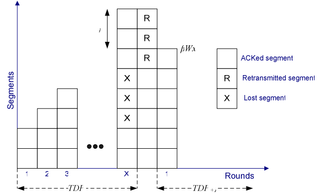
Fig. 5. Evolution of SAIMD TCP Sack congestion window over OBS networks.
