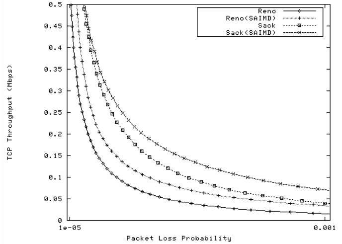
Fig. 11. Throughput of TCP Reno/Reno(SAIMD), TCP Sack/Sack(SAIMD) in OBS with burst retransmission.
