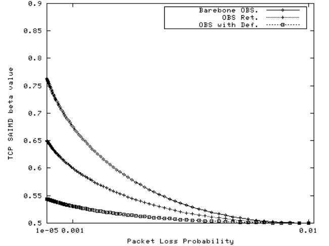
Fig. 8. Segment loss probability vs. the average values of \beta in the SAIMD scheme.
