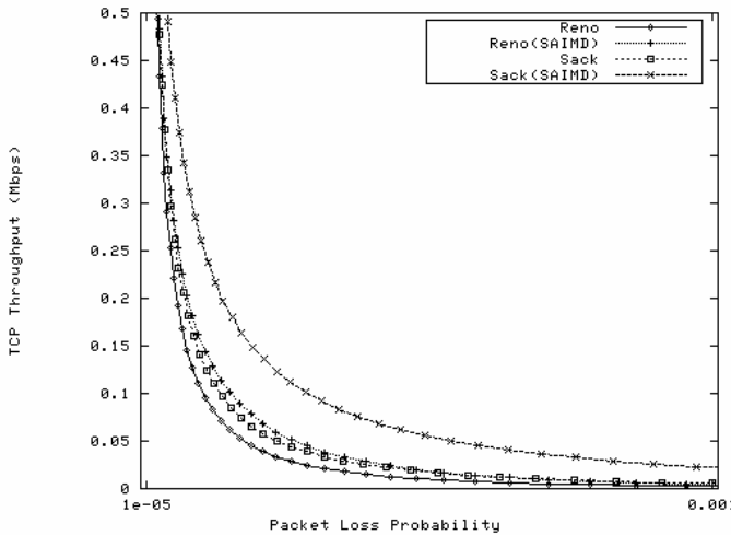
Fig. 10. Throughput of TCP Reno/Reno(SAIMD), TCP Sack/Sack(SAIMD) in the barebone OBS network.
