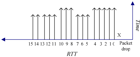
Fig. 2. Numbering of RTTs, where RTT(0) denotes the RTT right before a segment loss occurs.
