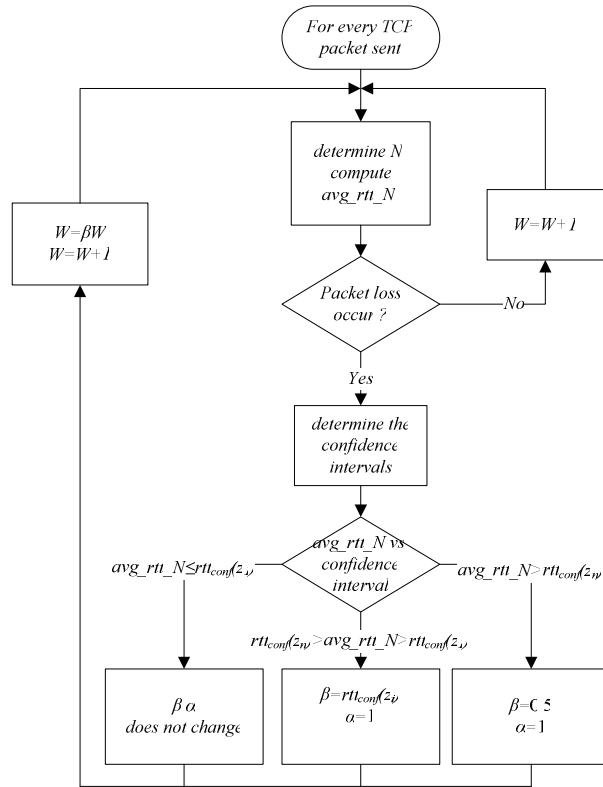
Fig. 4. The proposed SAIMD congestion control scheme.
