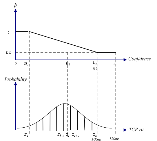
Fig. 3. The relation of z_i , u_i , and \beta in the SAIMD scheme.
