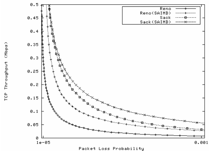
Fig. 12. Throughput of TCP Reno/Reno(SAIMD), TCP Sack/Sack(SAIMD) in the OBS network with burst deflection.
