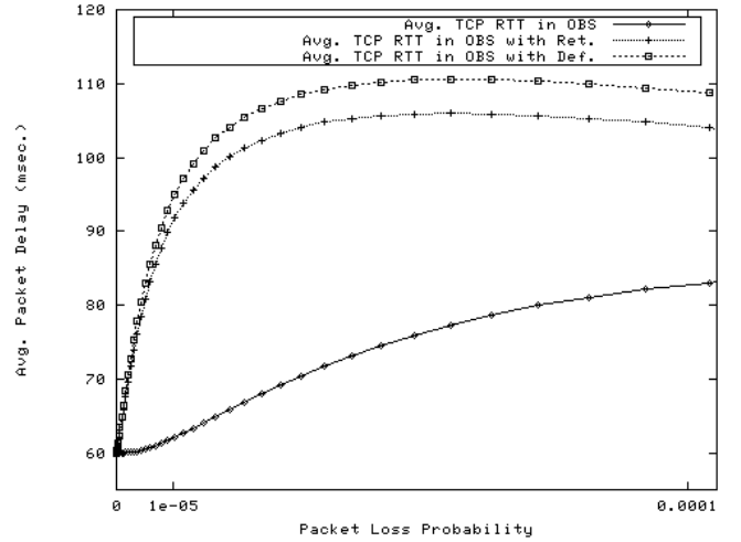
Fig. 7. Average TCP RTT vs. segment loss probability.
