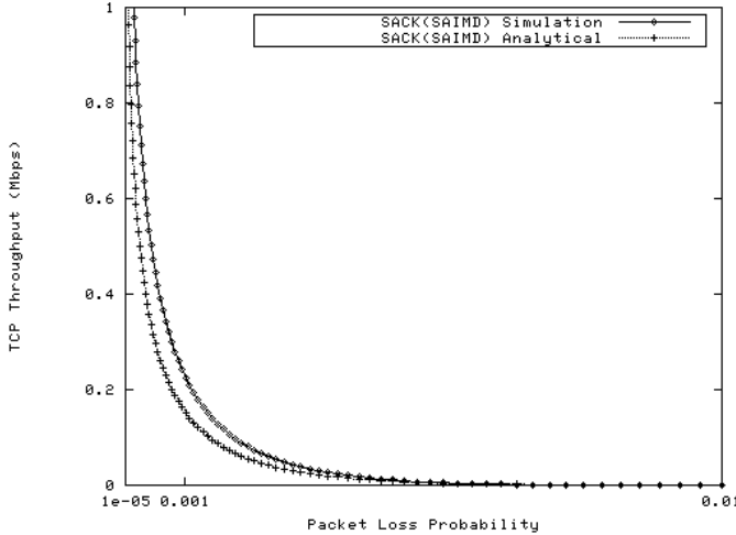
Fig. 9. SAIMD throughput from the simulation model vs. the analytical model.
